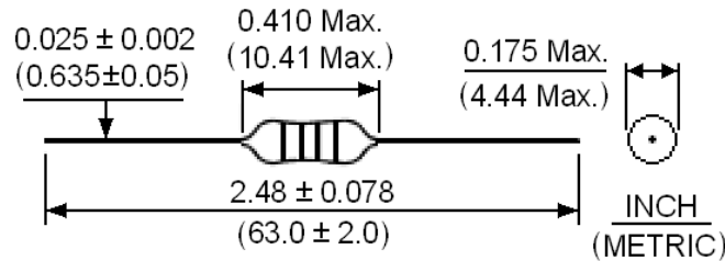
Mechanical drawing
