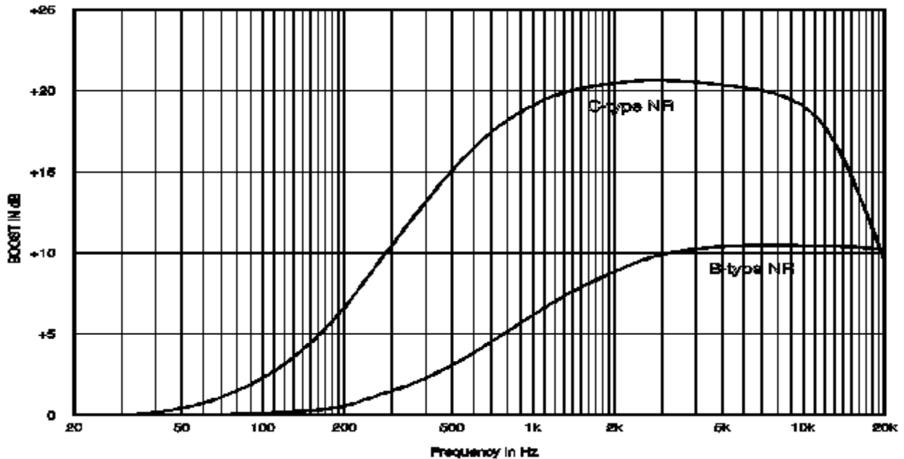
Figure 6. Low-level encoding characteristics of Dolby B and Dolby C. More boost is provided by Dolby C, and it extends about two octaves lower. The playback decoding, and thus the maximum noise reduction effect, is the reciprocal of the curves shown.
