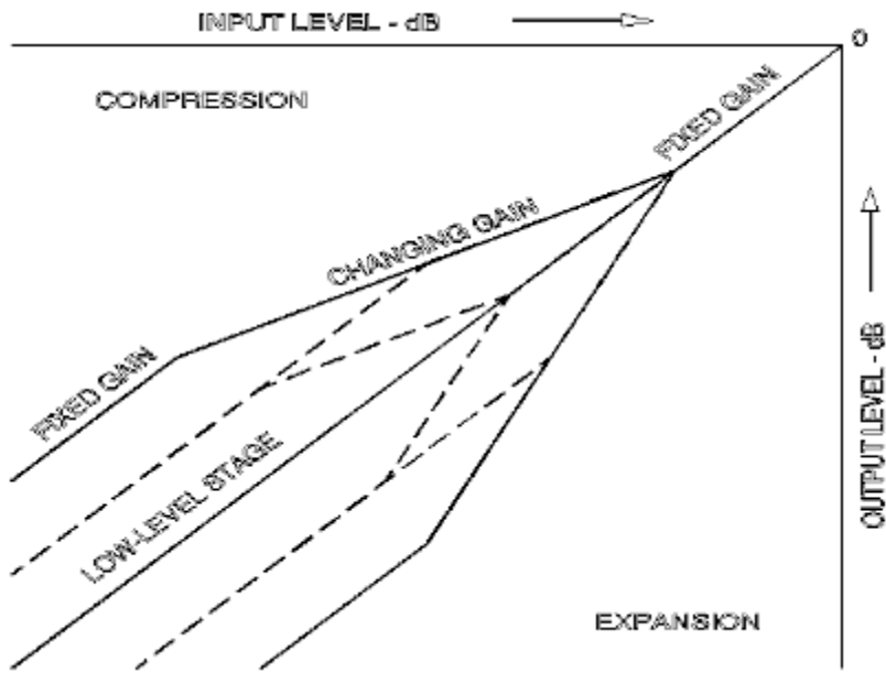
Figure 8. The Dolby S-type NR system prevents multiplication of compression ratios by staggering the signal levels at which gain changes occur, as shown for the high-level stage (A) and low-level stage (B). However, at low levels, the boost of the two stages add (C) to provide more noise reduction.
