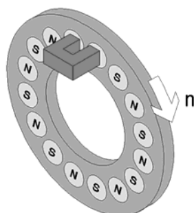
Figure 2: basic principle of AXIFUS
