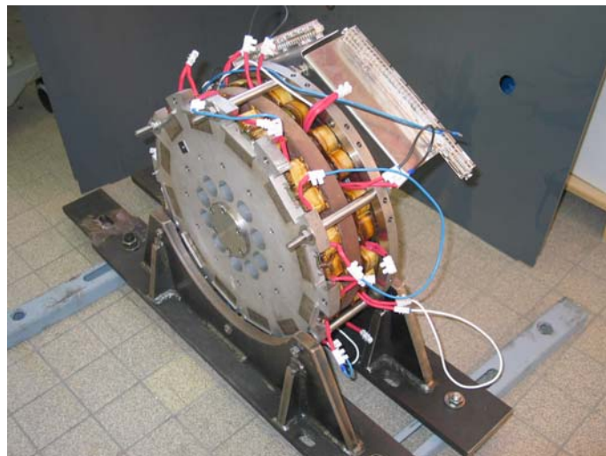
Figure 1: Assembled Axifus generator
