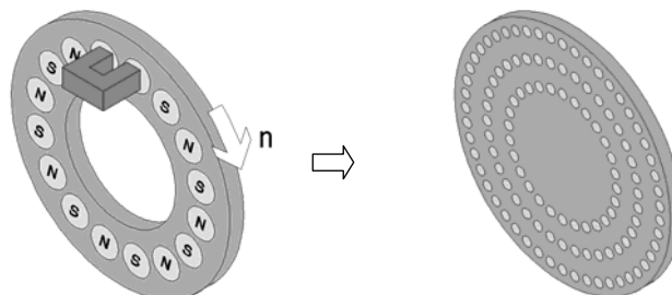
Figure 4: basic principle of AXIFUS to the principle of using magnets on more than 1 rotor radius
