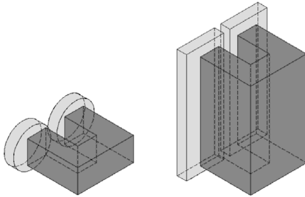
Figure 3: configuration with cylindrical permanent magnets and with rectangular ones
