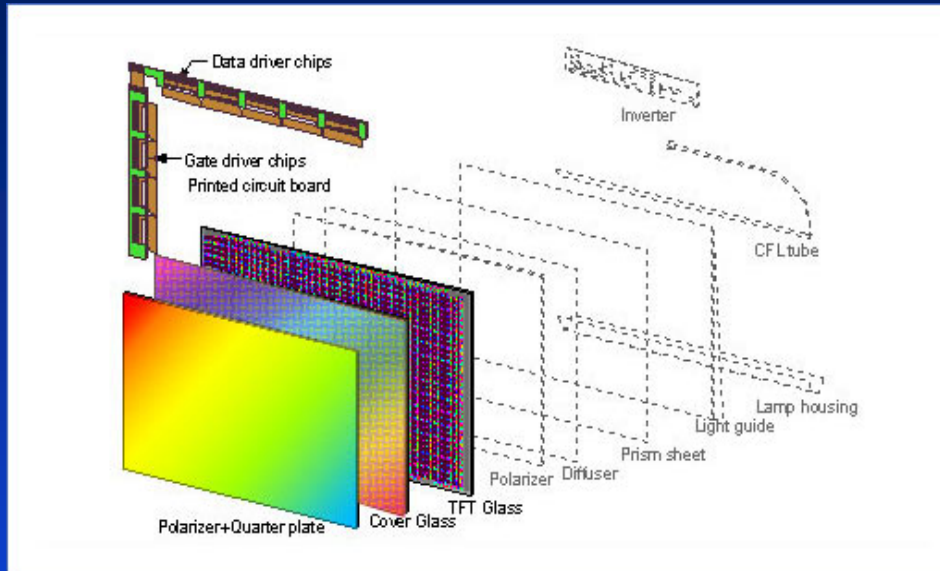
Figure 1 - AMOLED
