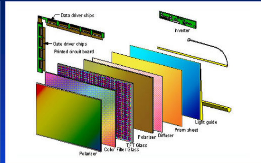
Figure 2 – TFT Display
