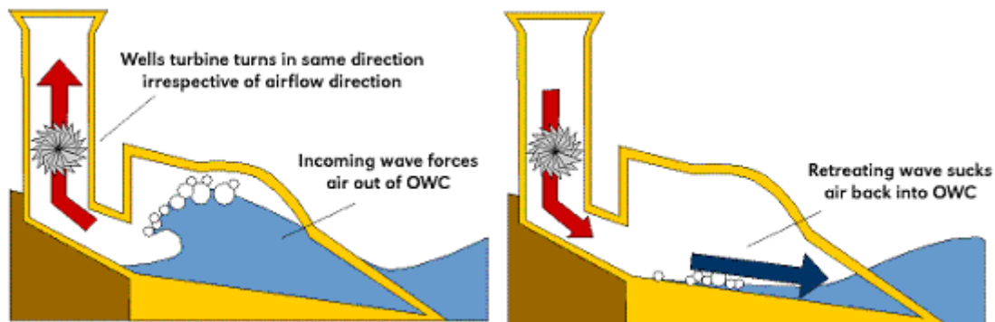
Figuur 20: Oscillating Water Column (OWC)
