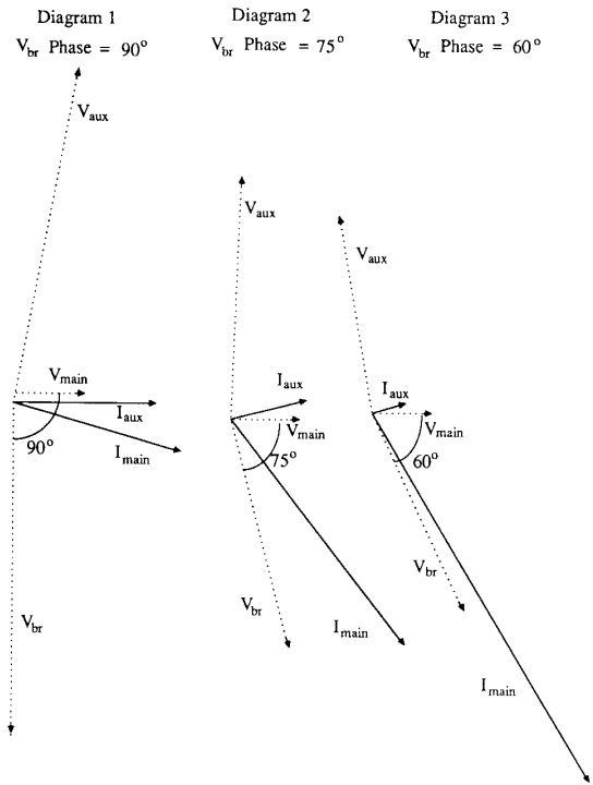
Fig. 4. Phasor diagrams for capacitor bridge run machine at rated torque for bridge phase angles of 90, 75, and 60°.
