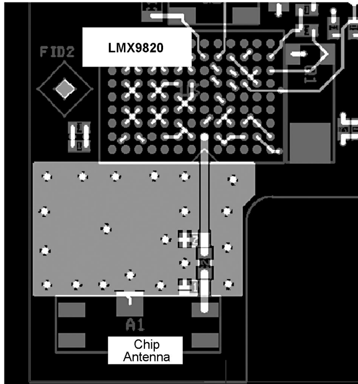
FIGURE 36. Ceramic Chip Antenna for Distance Meter
