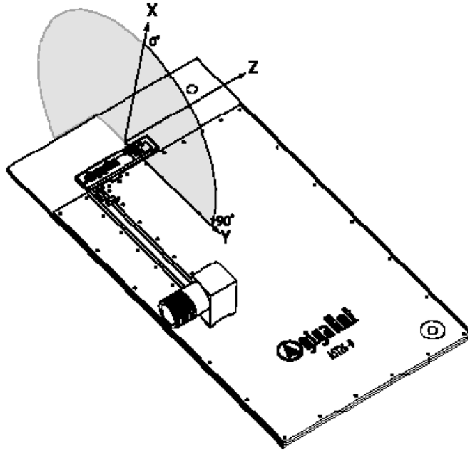
FIGURE 41. GigaAnt Rufa 2.4 GHz SMD Antenna
