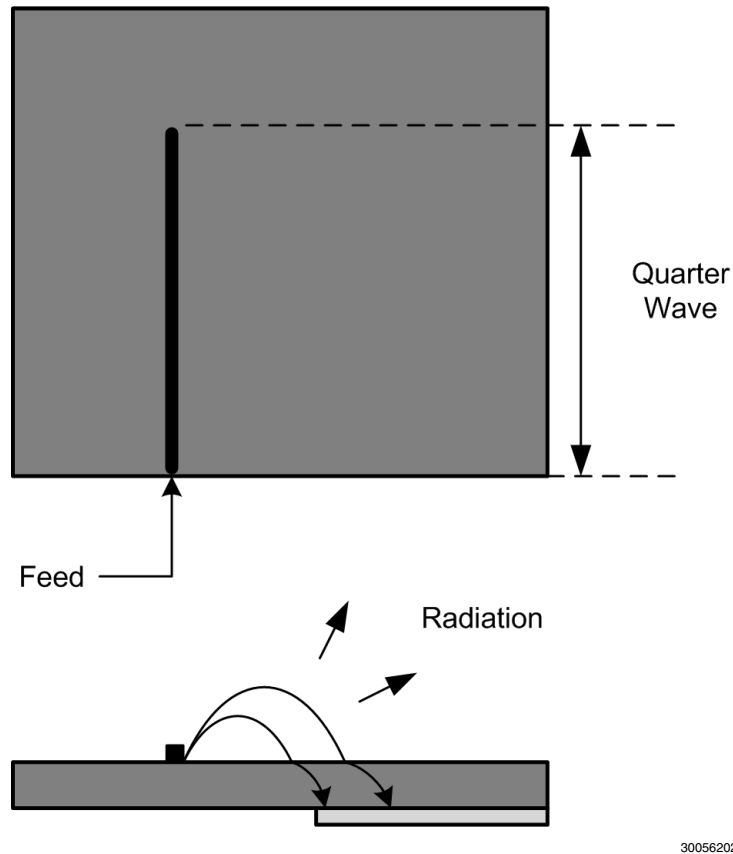
FIGURE 2. Fringing Field With Partial Ground Plane
