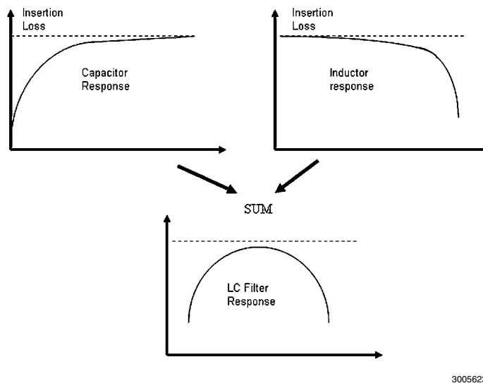
FIGURE 30. LC Filter Response
