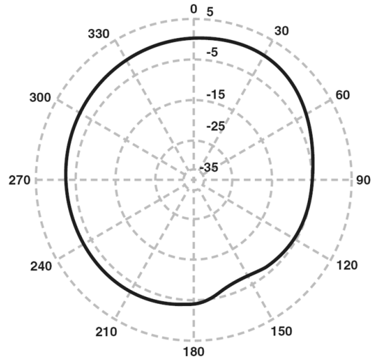
Elevation Cut
