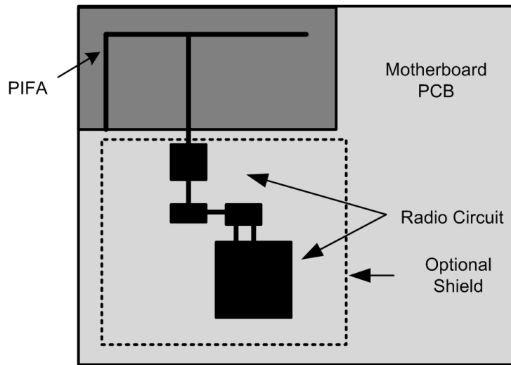
FIGURE 6. PIFA Antenna Placement
