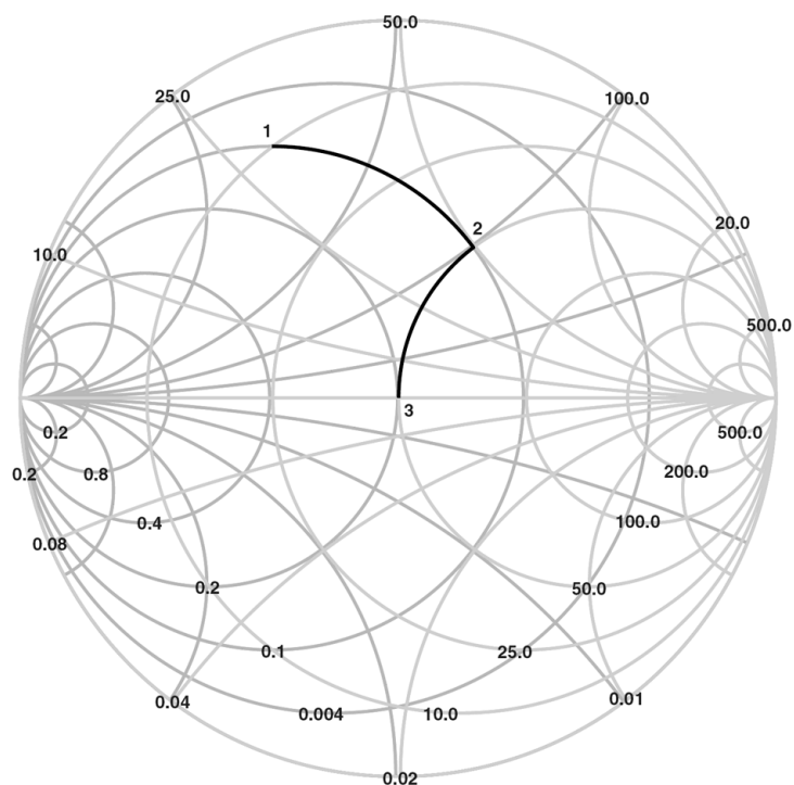
FIGURE 22. After Conductance-Resistance Tuning
