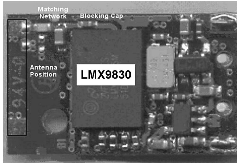
FIGURE 13. LMX9830 Antenna
