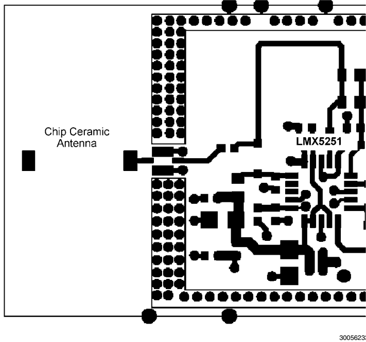
FIGURE 33. Ceramic Chip Antenna for Industrial Remote Control with External PA
