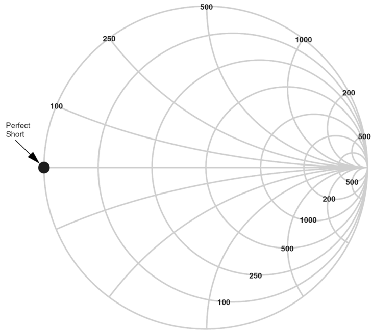
FIGURE 15. Smith Chart, Perfect Short
