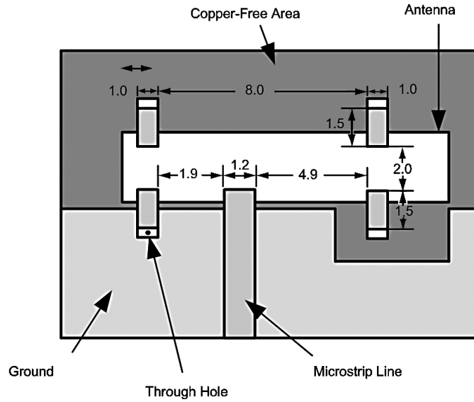
FIGURE 9. Typical Chip PCB Footprint
