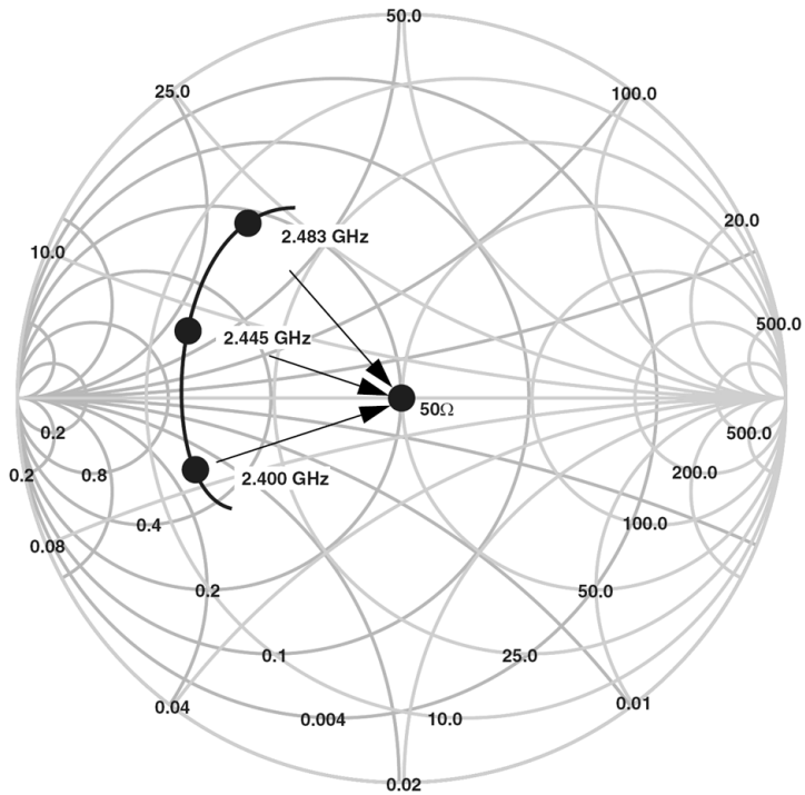
FIGURE 24. Broadband Match
