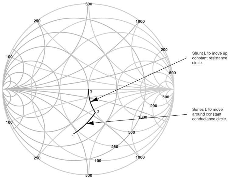
FIGURE 18. Impedance Transformation
