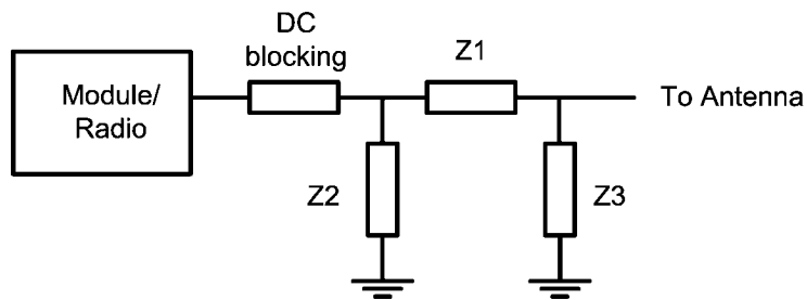
FIGURE 25. PI Network
