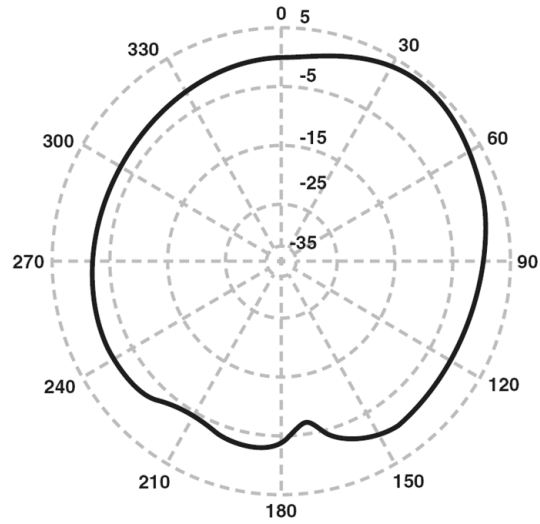
Azimuth Cut
