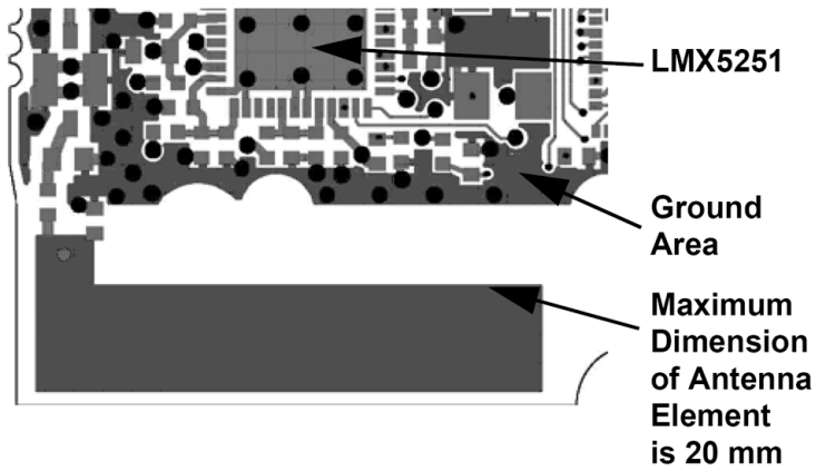
FIGURE 10. LMX5251 PIFA Antenna
