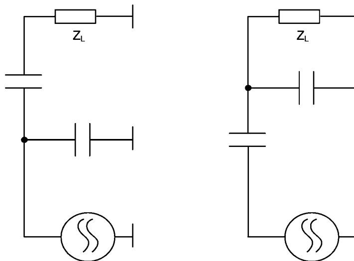
FIGURE 23. Two Possible Matching Networks
