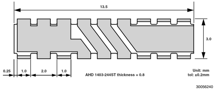
FIGURE 40. Surface-Mount Chip Antenna (Mitsubishi Materials AHD 1403) for Electronic Whiteboard
