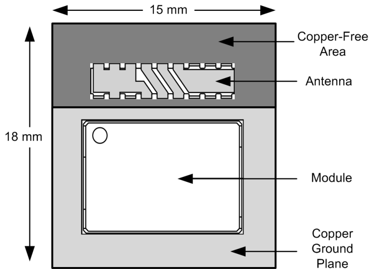
FIGURE 12. LMX9820A Antenna
