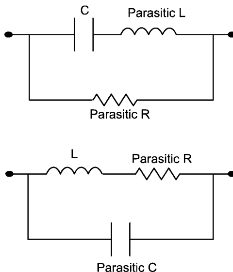
FIGURE 26. Component Models
