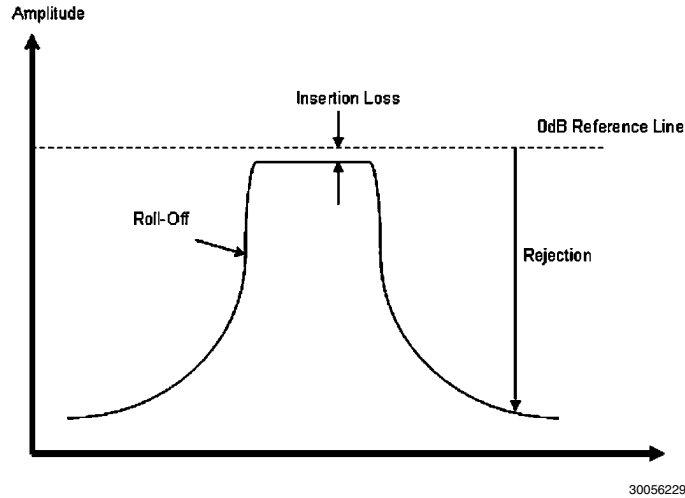
FIGURE 29. RF Filter Performance
