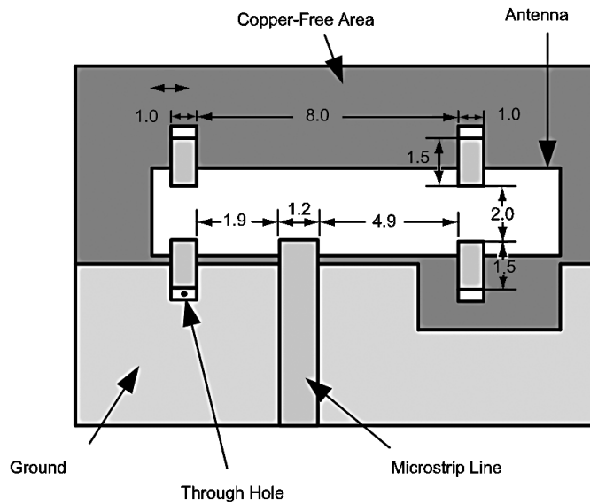
FIGURE 42. Mitsubishi AHD1403 Surface-Mount Antenna
