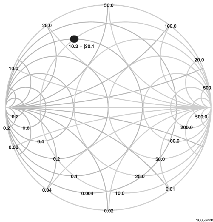
FIGURE 20. Single Frequency Data Point
