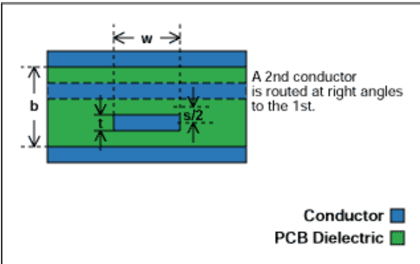
Figure 4. Dual orthogonal stripline.
