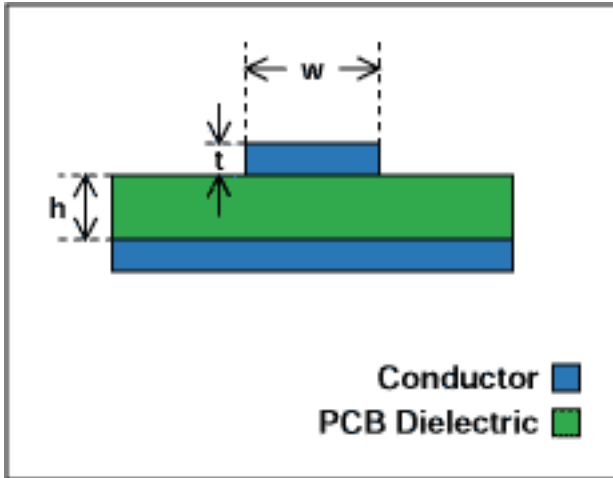
Figure 5. Microstrip line.
