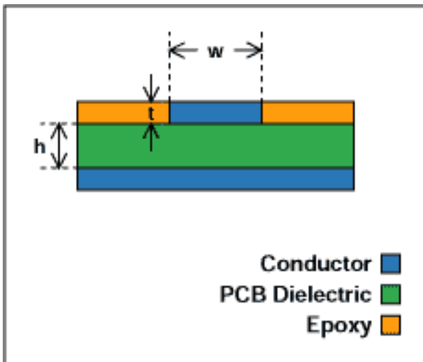
Figure 6. Embedded microstrip line.
