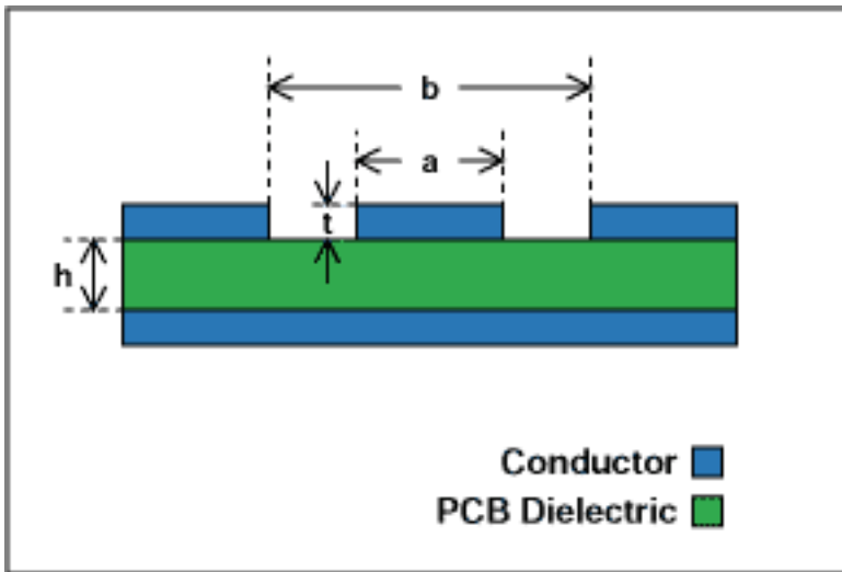
Figure 9. Coplanar waveguide with ground.
