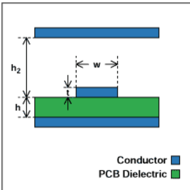
Figure 7. Covered microstrip line.
