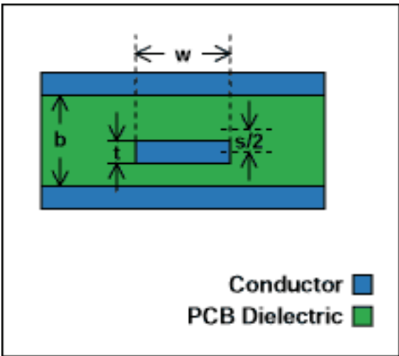
Figure 3. Off-center stripline.
