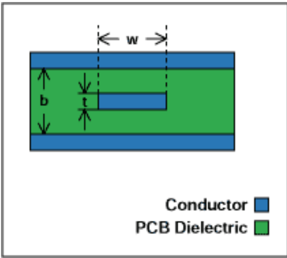
Figure 2. Centered stripline.
