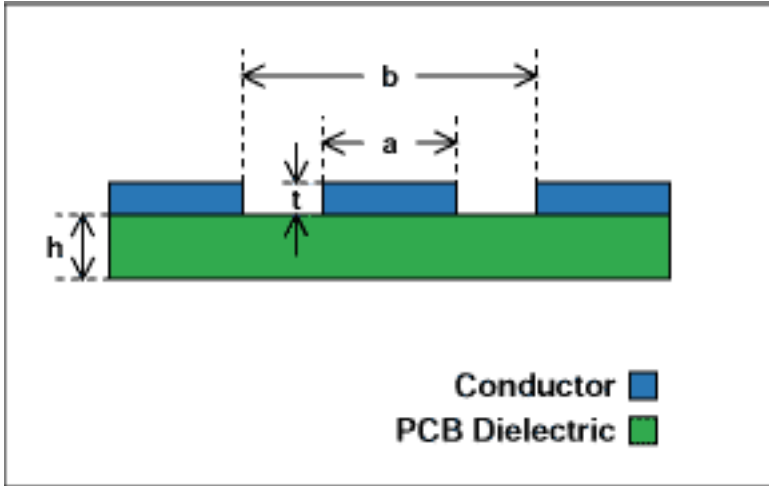
Figure 8. Coplanar waveguide.
