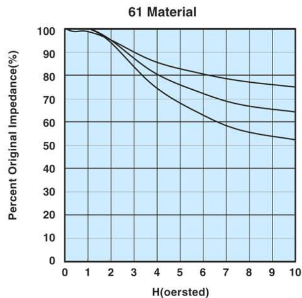
Figure 23 Percent of Original Impedance vs. Magnetic Field Strength. Measured on a 2661000301 using the HP4291A.
