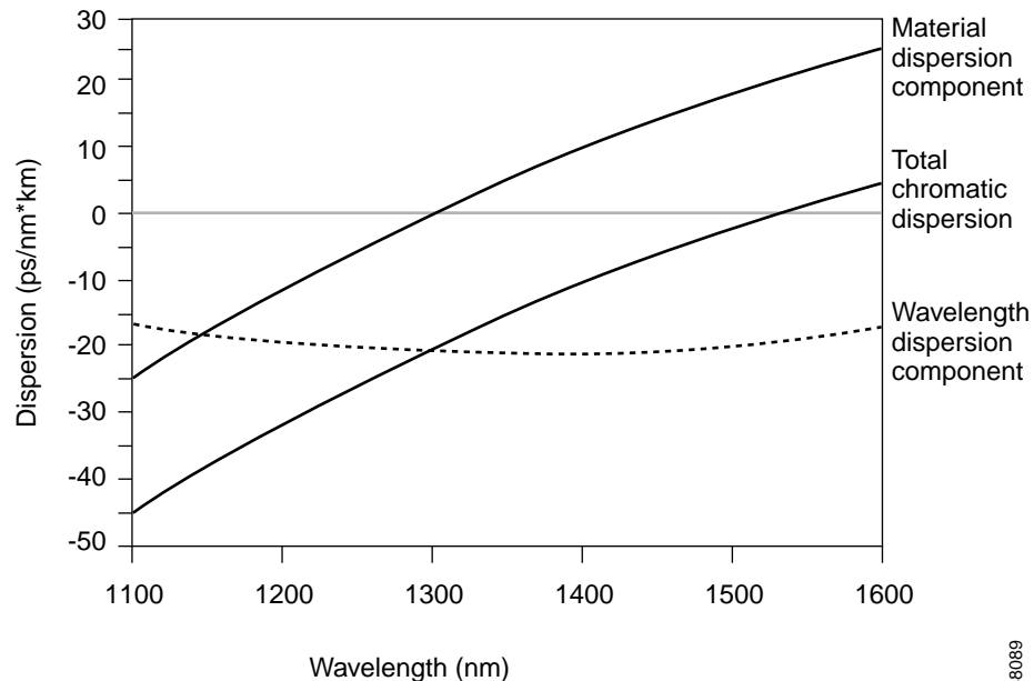
Figure 2-13 Chromatic Dispersion
