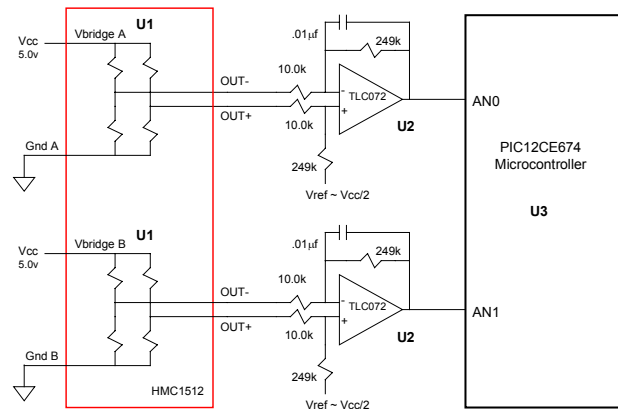
Figure 10 HMC1512 Circuit
