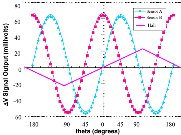
Figure 18 360° Sensing Waveform
