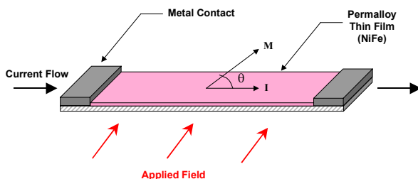
Figure 1 AMR Element
