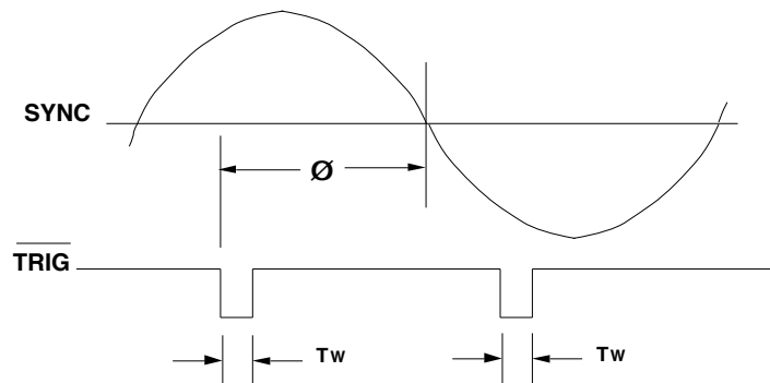
FIGURE 3. TRIG OUTPUT CONDUCTION ANGLE, Ø
