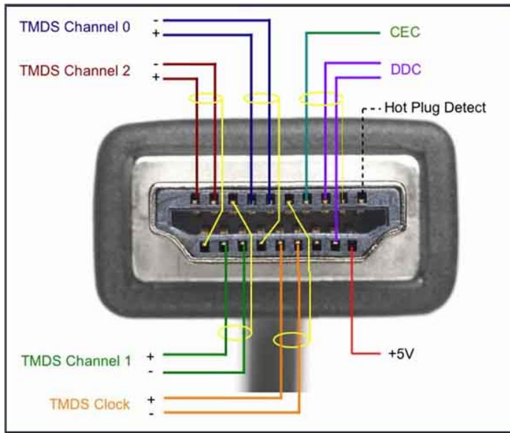
Cross Section of HDMI Connector
