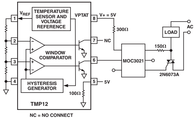
Figure 14. Controlling the 2N6073A Triac
