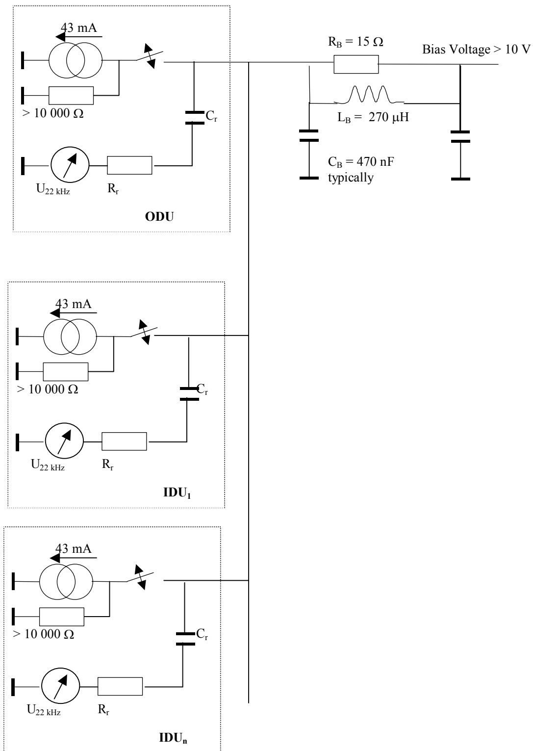
Figure 10.2: 22 kHz PWK bus concept
