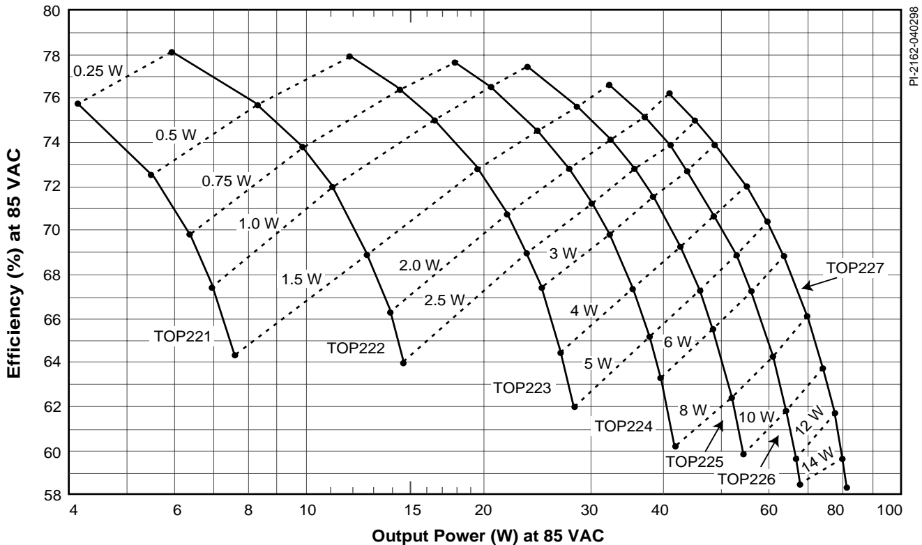
Figure 3. Typical Efficiency vs Output Power with Contours of Constant TOPSwitch-II Power Loss for Universal Input and 5 V Output.
