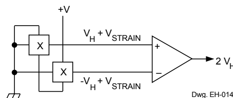
Multiple Devices to Cancel Effects of Strain
