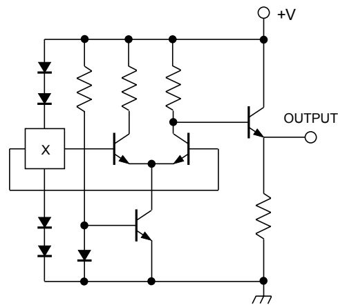
Early Linear Ratiometric Device Using Single Hall Element
