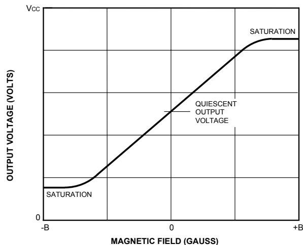
Linear Device Characteristic
