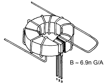
Multiple Turns for Measuring Low Currents
