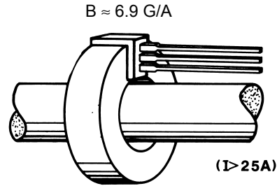
Gapped Toroid for Measuring High Currents
