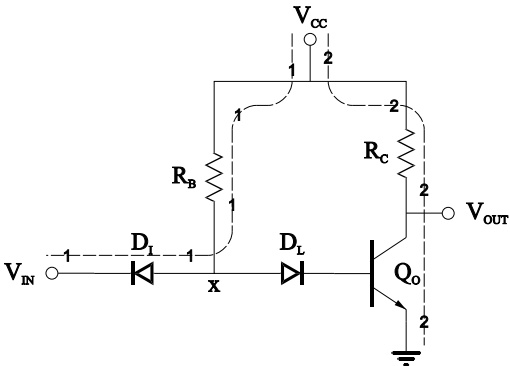
Basic Inverter
