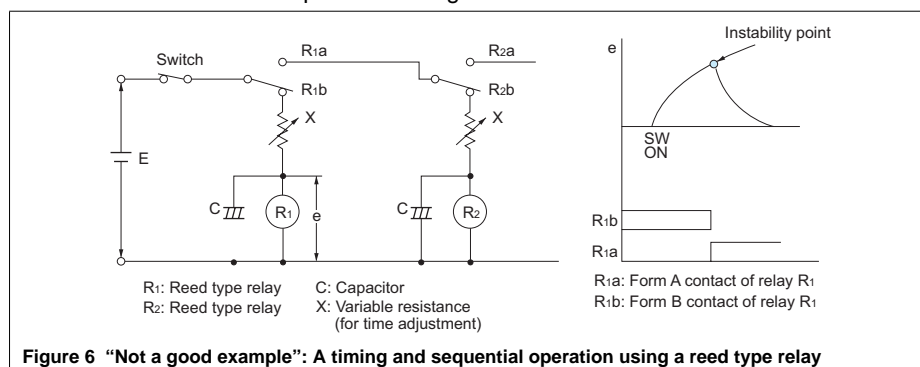
Figure 6 "Not a good example": A timing and sequential operation using a reed type relay
