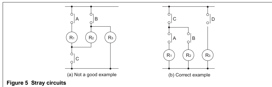
Figure 5 Stray circuits
