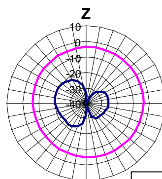
GAIN[dBi]
