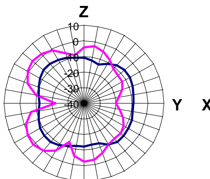
GAIN[dBi]
