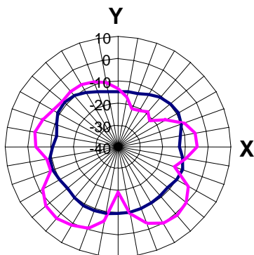
GAIN[dBi]
