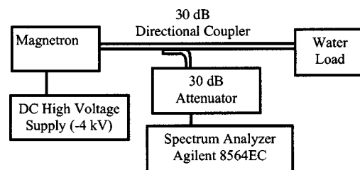
FIG. 1. Experimental configuration for oven magnetron spectrum analysis.
