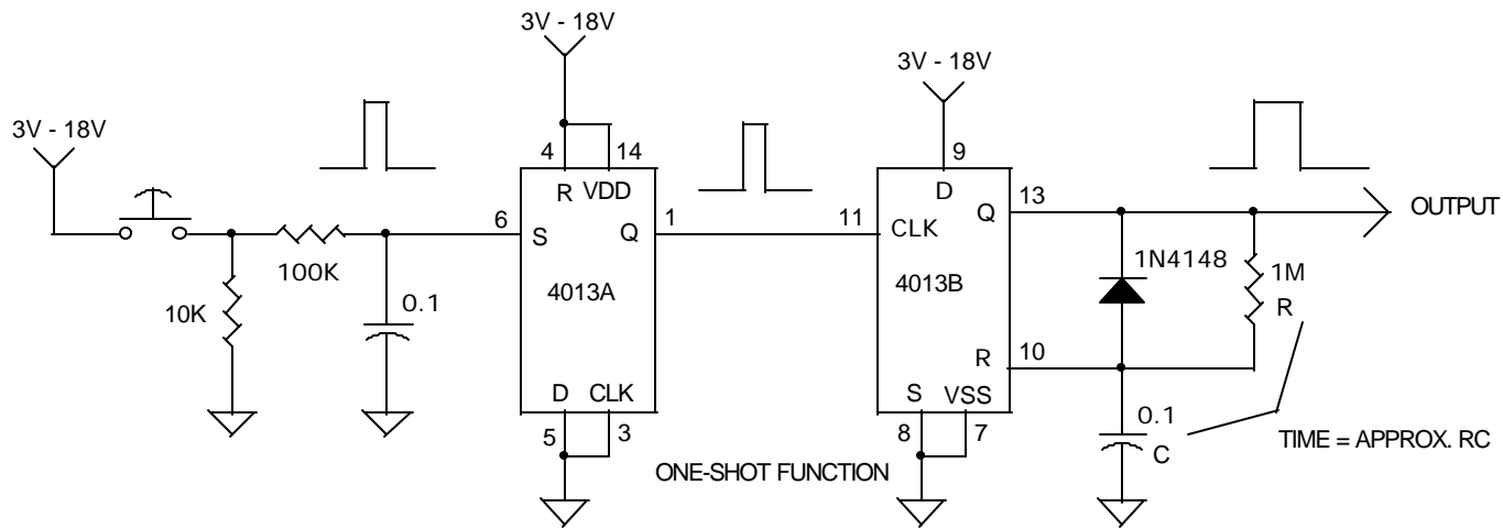
ONE PULSE GENERATED WITH EACH PUSH OF THE BUTTON OR ANY POSITIVE PULSE
