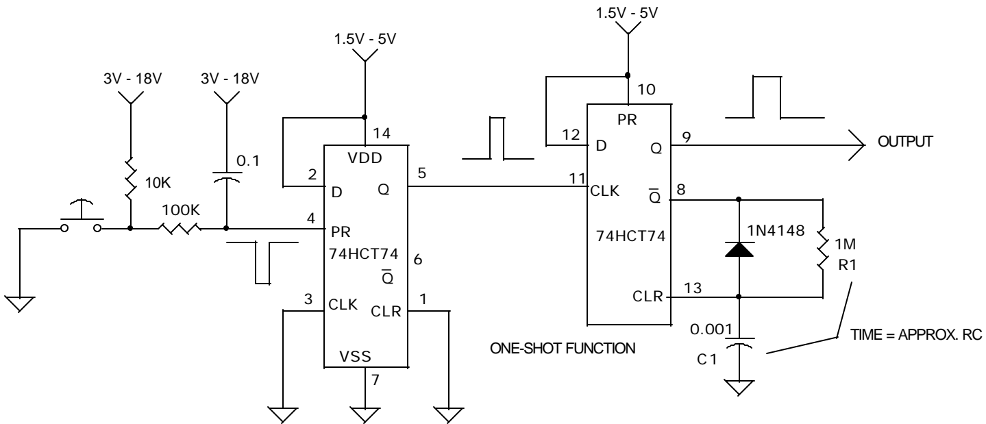
ONE PULSE GENERATED WITH EACH PUSH OF THE BUTTON OR ANY NEGATIVE PULSE
