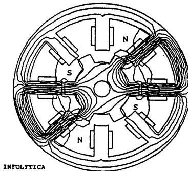
FIG. 9B CONVENTIONAL VRBLDC
