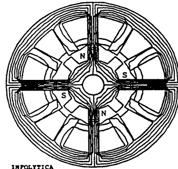
CONVENTIONAL VRBLDC
