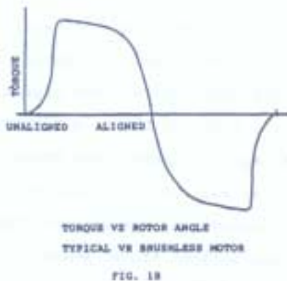
Fig. 1A shows the typical torque per step of a VR stepping motor and Fig. 1B shows the torque curve of a single "stroke" of a somewhat typical VR brushless motor. (Both examples have one phase energized per step or per stroke.)
