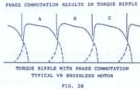
Fig. 2A and 2B show the torque production with subsequent phases energized. The torque ripple is clearly evident. Note that this phenomenon is a motor characteristic not a control trait. Furthermore the torque ripple can be significantly altered with the control of current in each phase. (See Fig. A in Appendix)
