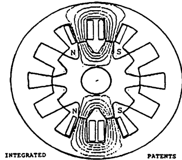
Fig. 8A NORMAL SATURATION
