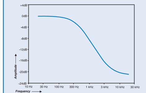
Figure 2-4b: de-emphasis in transmitter
