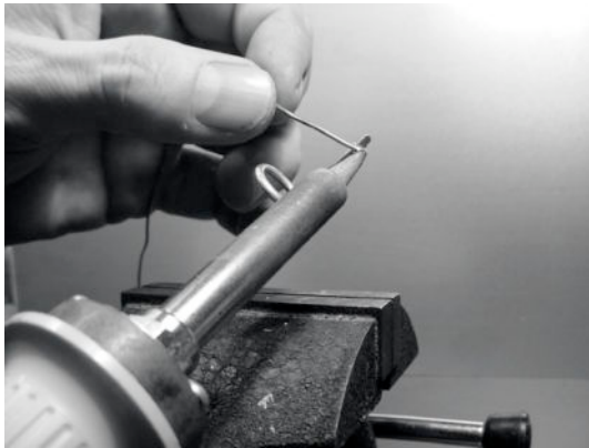
Figure 4.26: Add a little solder to the end of the wire to “tin” it prior to soldering.
